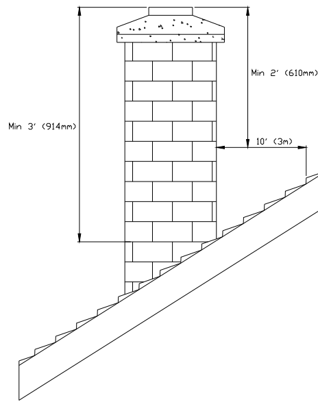
Figure 1.3 – Chimney height
