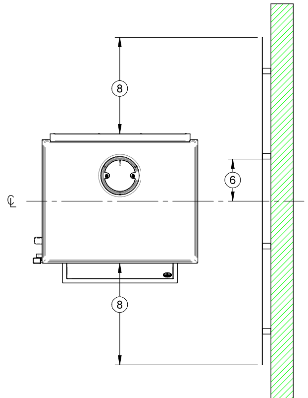
Figure 42: Clearances with Heat Shield - Top
