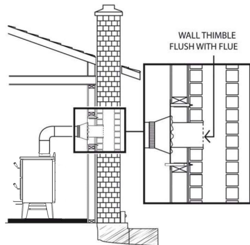
Figure 47: Masonry hearth installation
