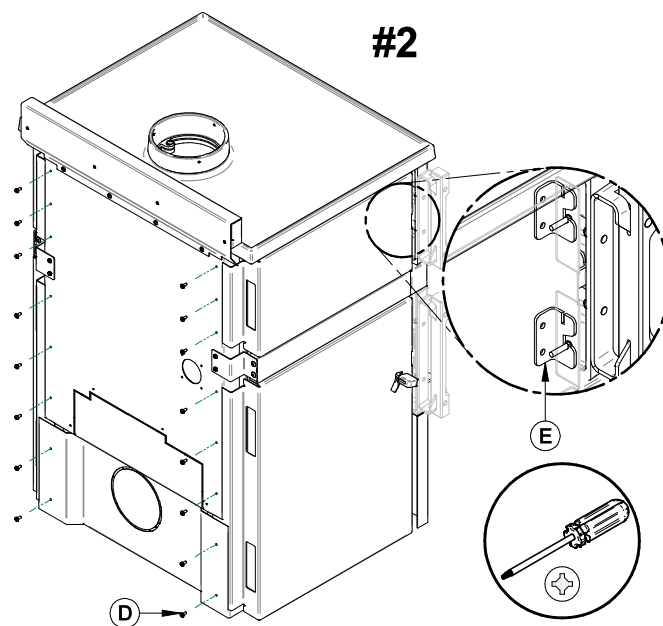
Figure 36: Decorative panels support
