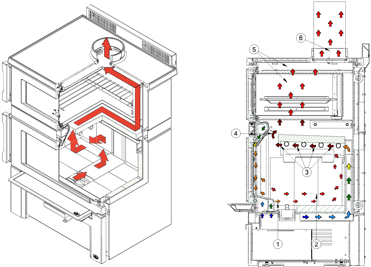
Figure 25: Gas path
