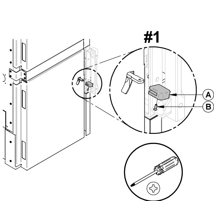
Figure 35: Remove the wooden handle
