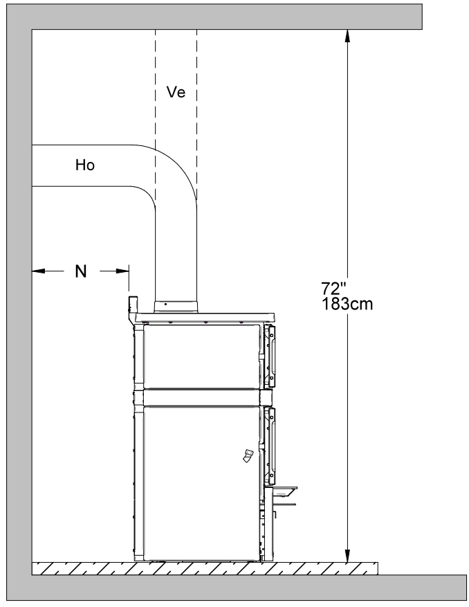
Figure 39: Clearances - Side
