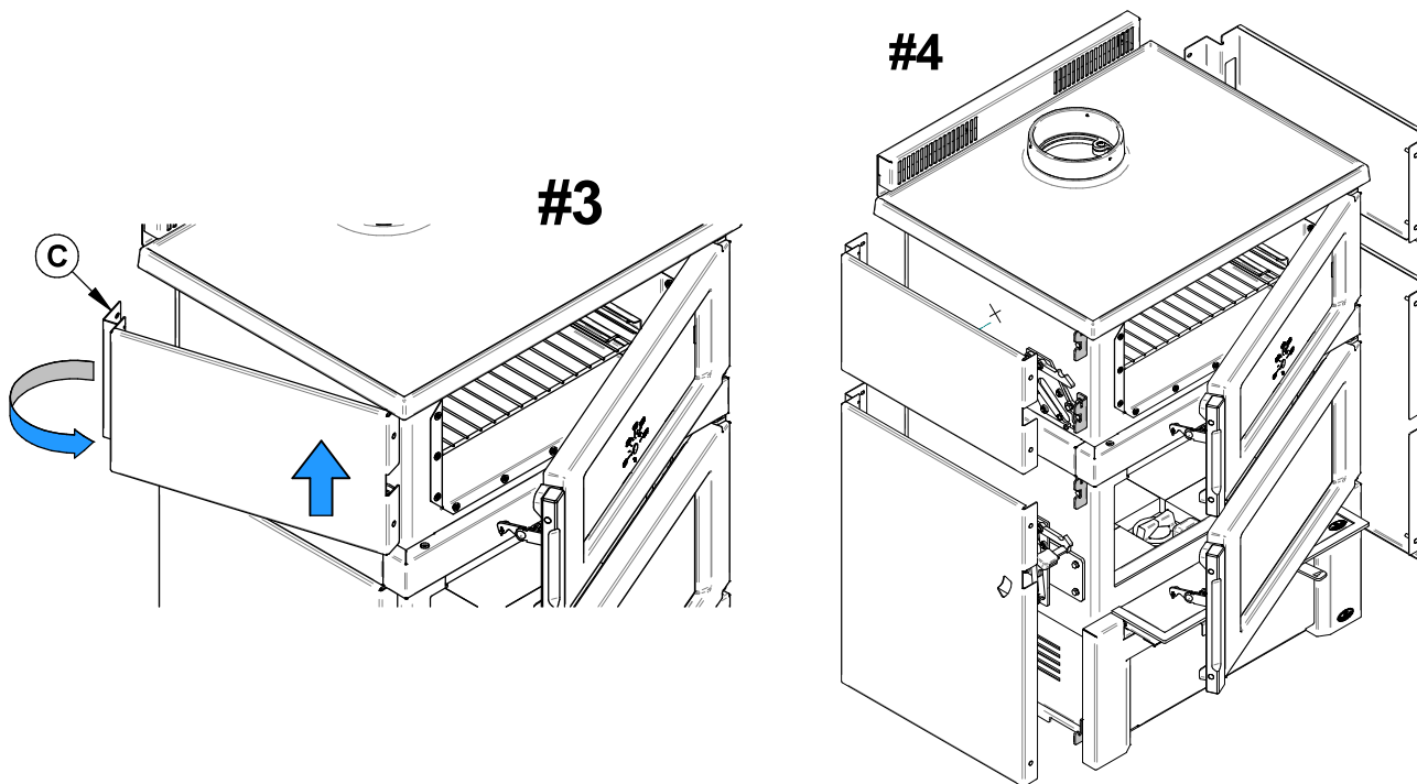
Figure 37: Remove the decorative panels
