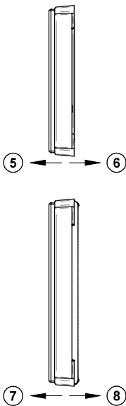
Figure 33: Eccentric hinges lateral adjustment
