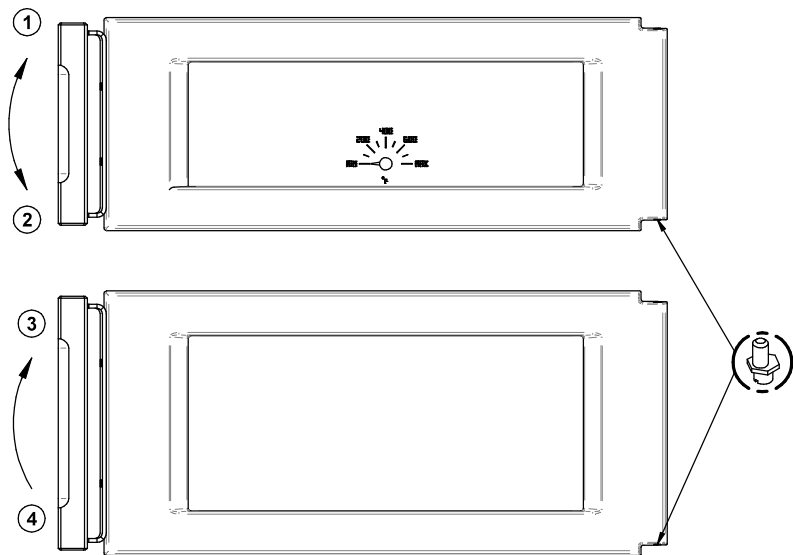
Figure 32: Doors adjustment
