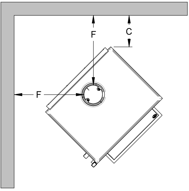
Figure 40: Clearances - Corner
