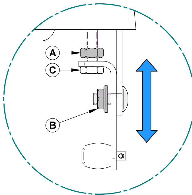
Figure 28: Oven door adjustment
