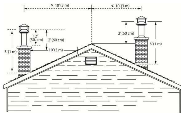
Figure 49: Sloping roof
