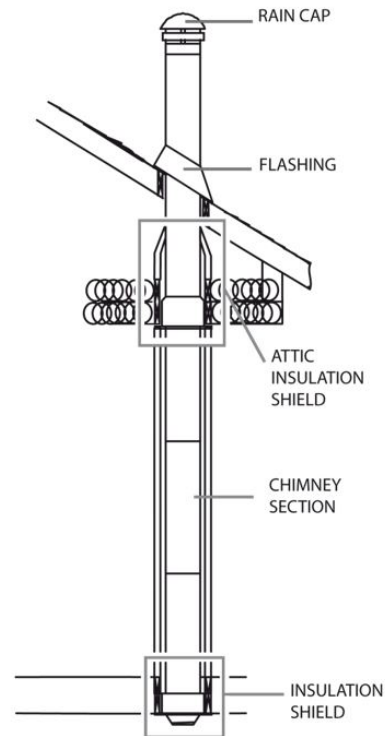
Figure 47: Standard installation
