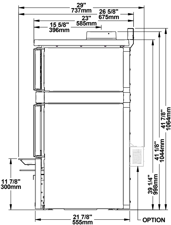
Figure 3: Side view
