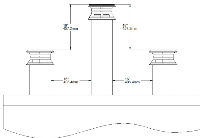
Figure 50: Flat roof
