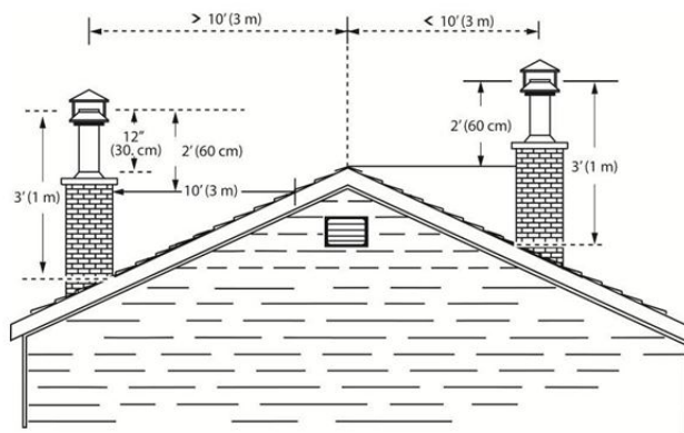
Figure 51: Sloping roof
