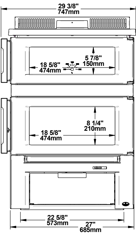
Figure 2: Front view
