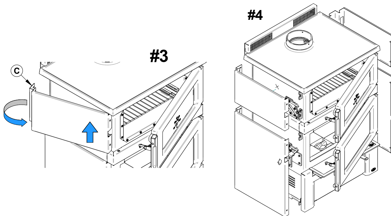
Figure 39: Remove the decorative panels
