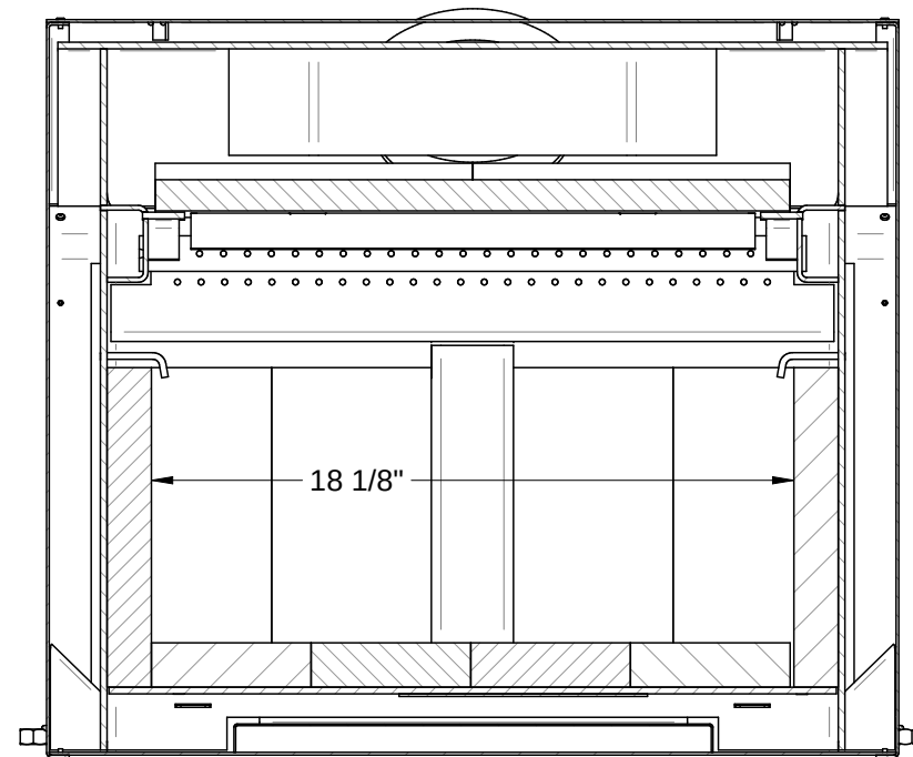
SECTION C-C
