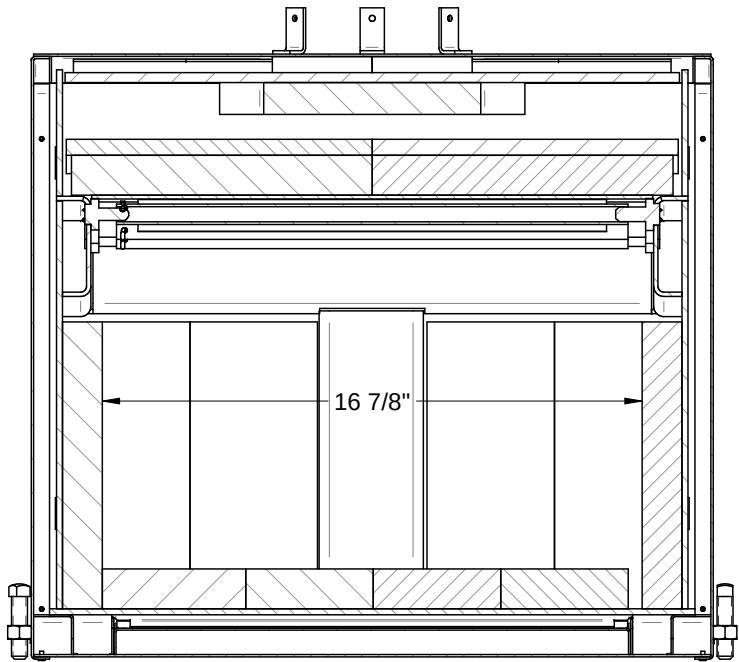
SECTION B-B
