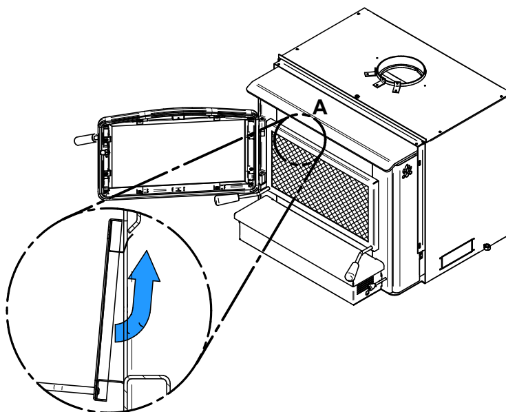
DETAIL A
