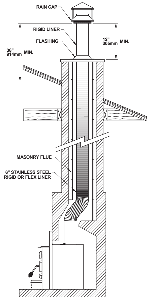
Figure 23: Liner Installation
