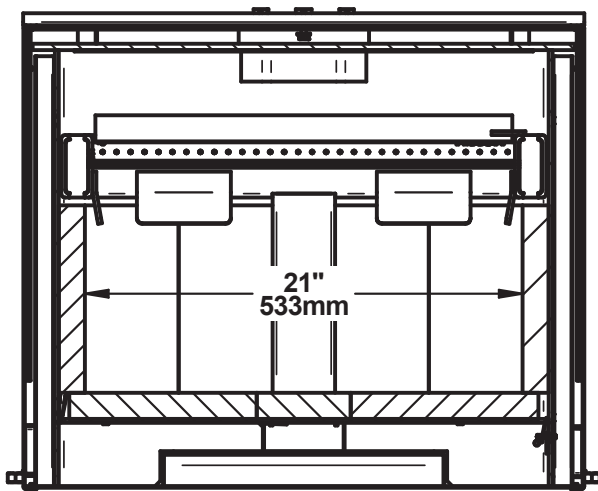
Figure 7: Front Firebox
