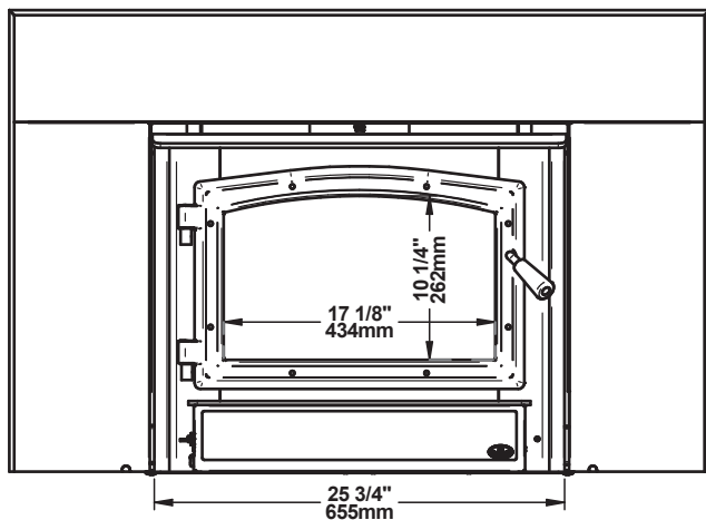
Figure 3: Front View
