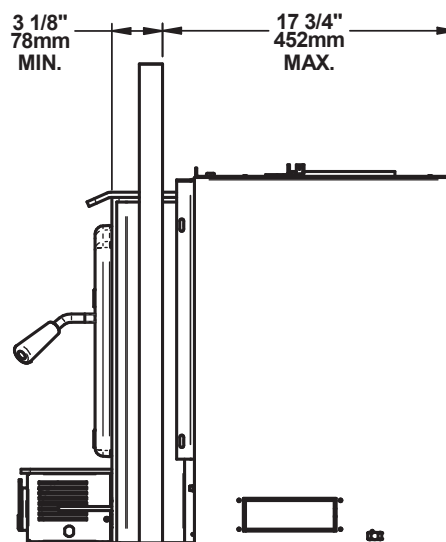
Figure 2: Side View - Minimum Insert Projection
