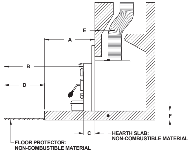
Figure 19: More than 5" raised base installation
