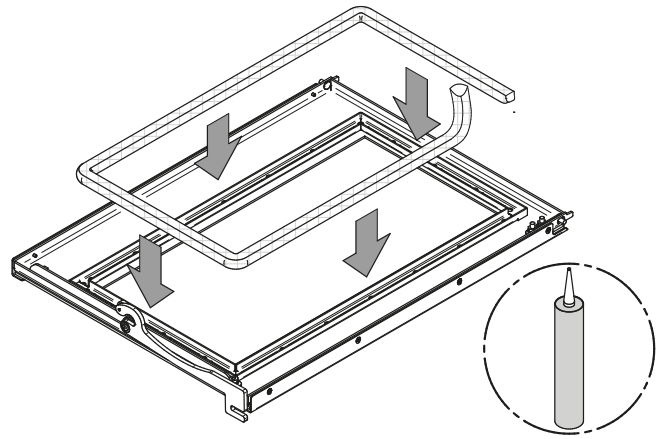
Figure 30: Door gasket
