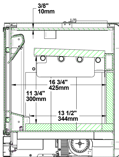
Figure 6: Side Firebox
