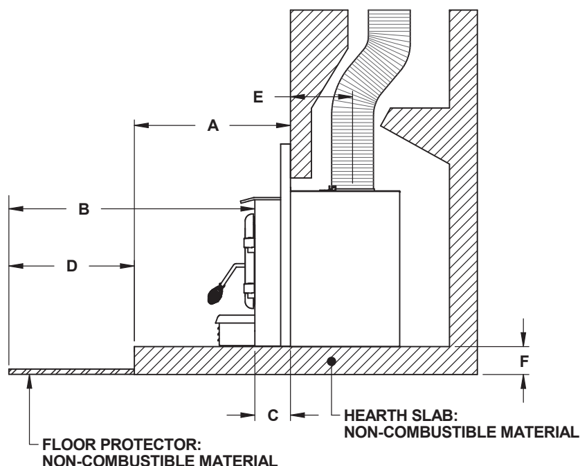
Figure 25: More than 5" raised base installation
