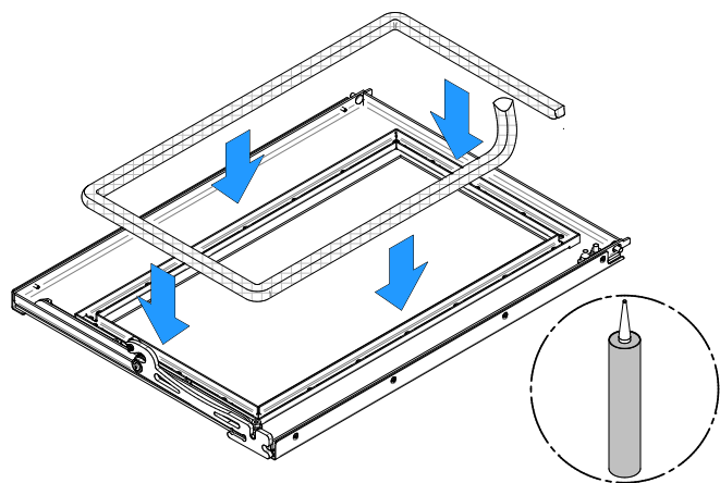
Figure 20: Door gasket
