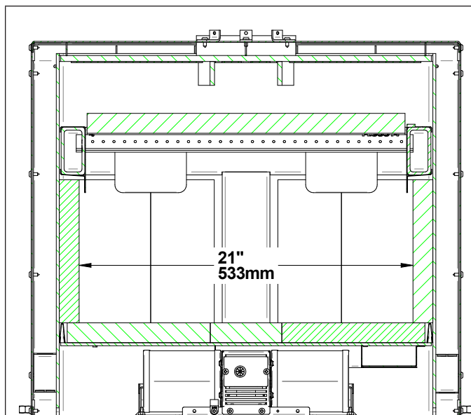
Figure 5: Front Firebox
