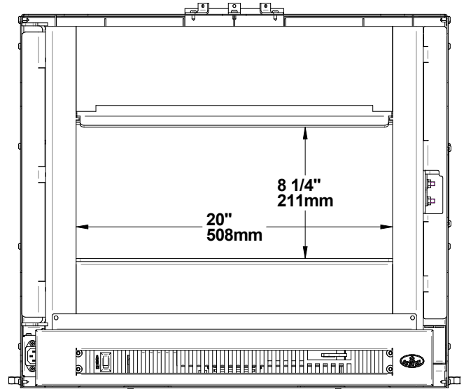
Figure 2: Door opening
