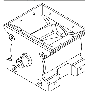
Rotative valve
