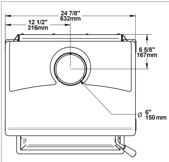
Figure 4: Top View
