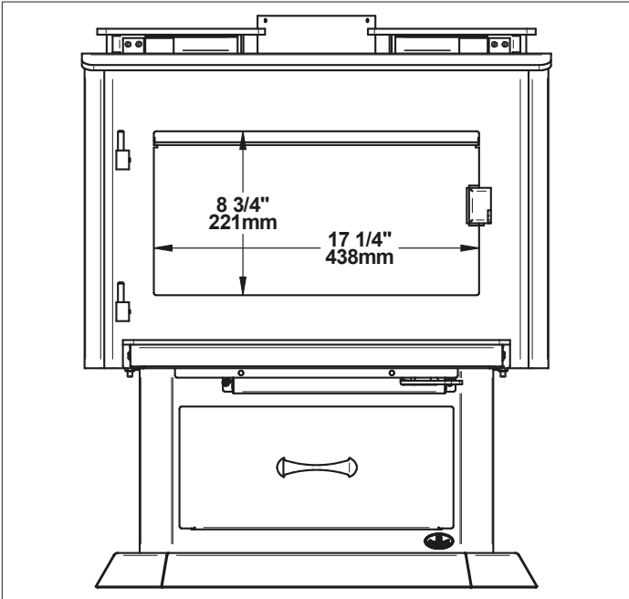
Figure 10: Door Opening
