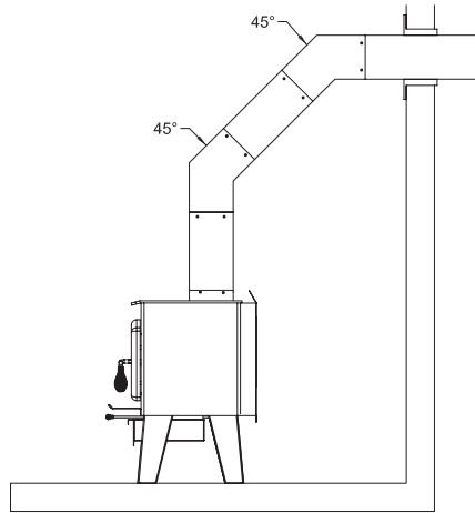
Figure 31: Acceptable
