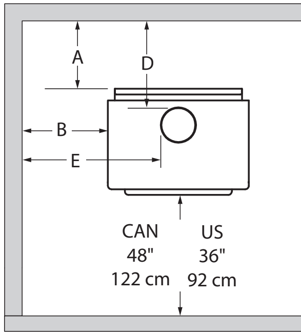
Figure 19: Clearances - Top
