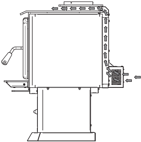
Figure 15: Air flow with a blower
