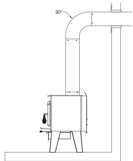
Figure 32: Avoid
