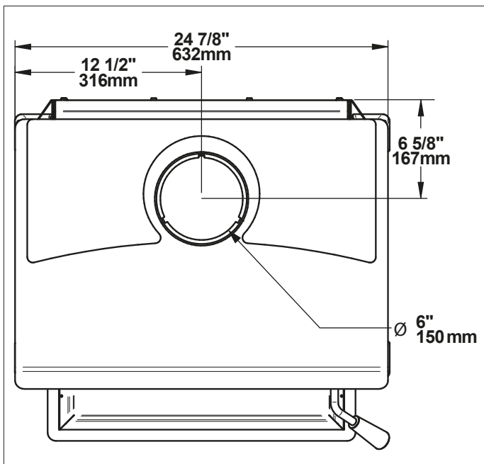
Figure 4: Top View
