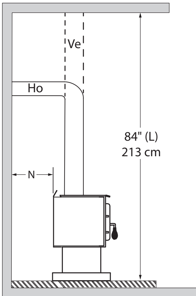
Figure 21: Clearances - Side
