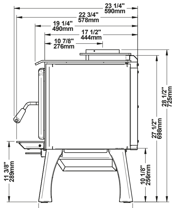
Figure 6: Side View
