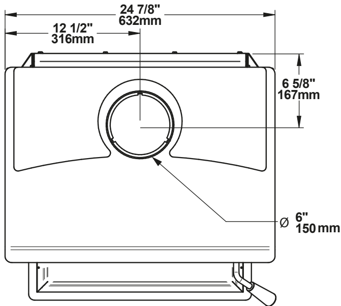
Figure 7: Top View
