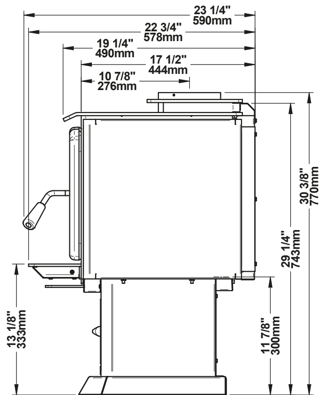
Figure 9: Side View
