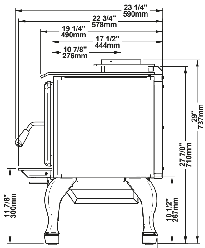
Figure 3: Side View
