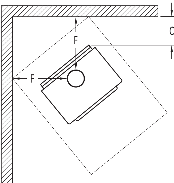
Figure 23: Clearances - Corner
