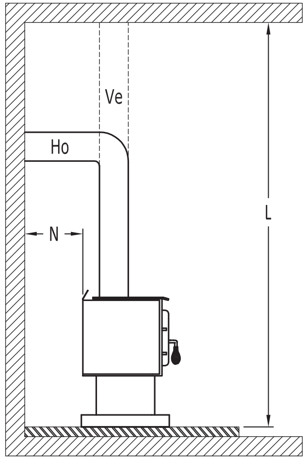
Figure 22: Clearances - Side
