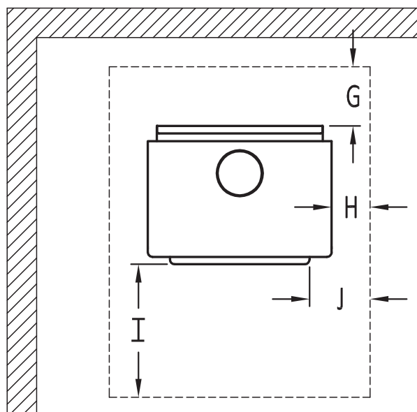
Figure 24: Floor Protection
