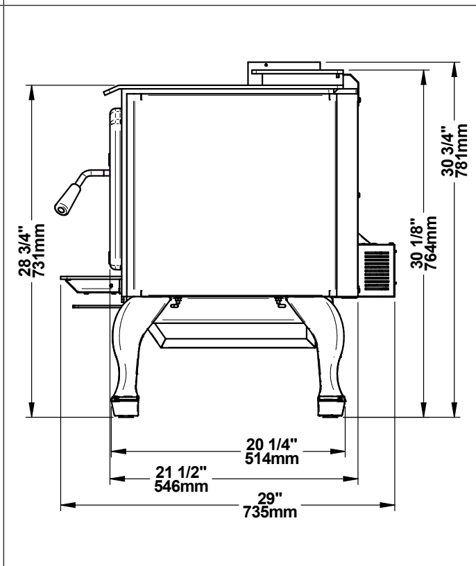
Figure 3: Side view
