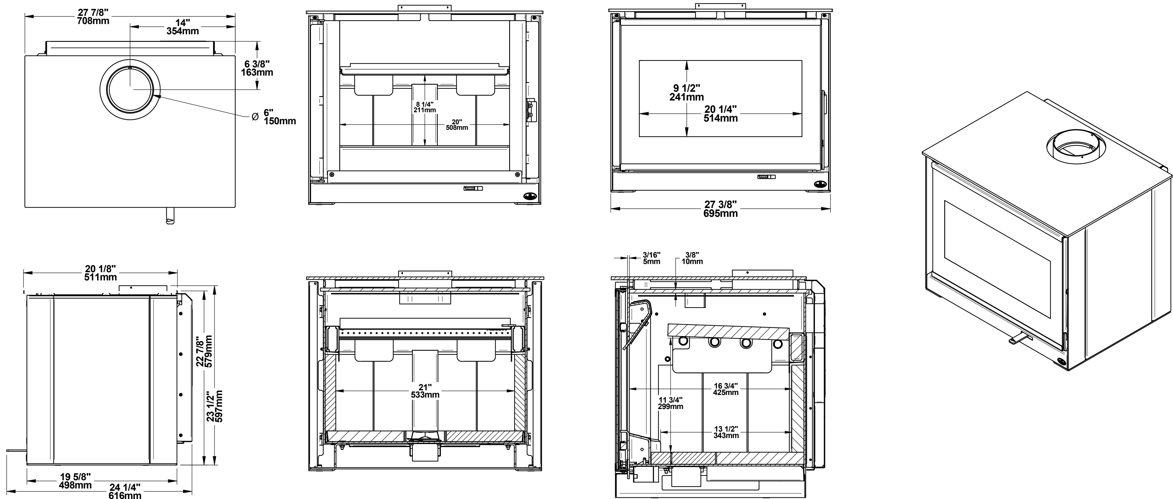
Base minimaliste / Minimalist base
