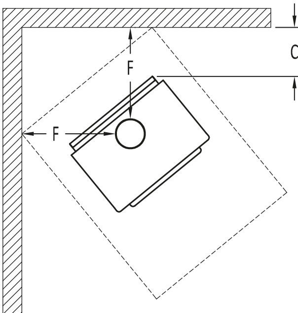
Figure 33: Clearances - Corner
