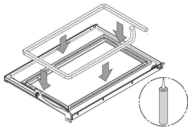
Figure 30: Door gasket
