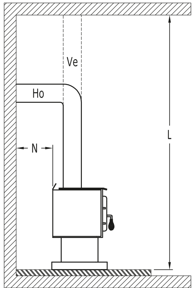
Figure 32: Clearances - Side
