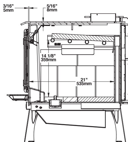
Combustion chamber - side view
