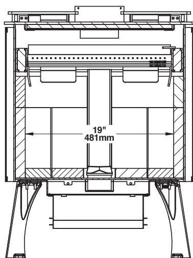
Combustion chamber - front view
