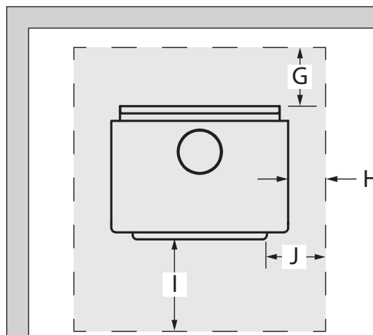
Figure 16: Floor Protection
