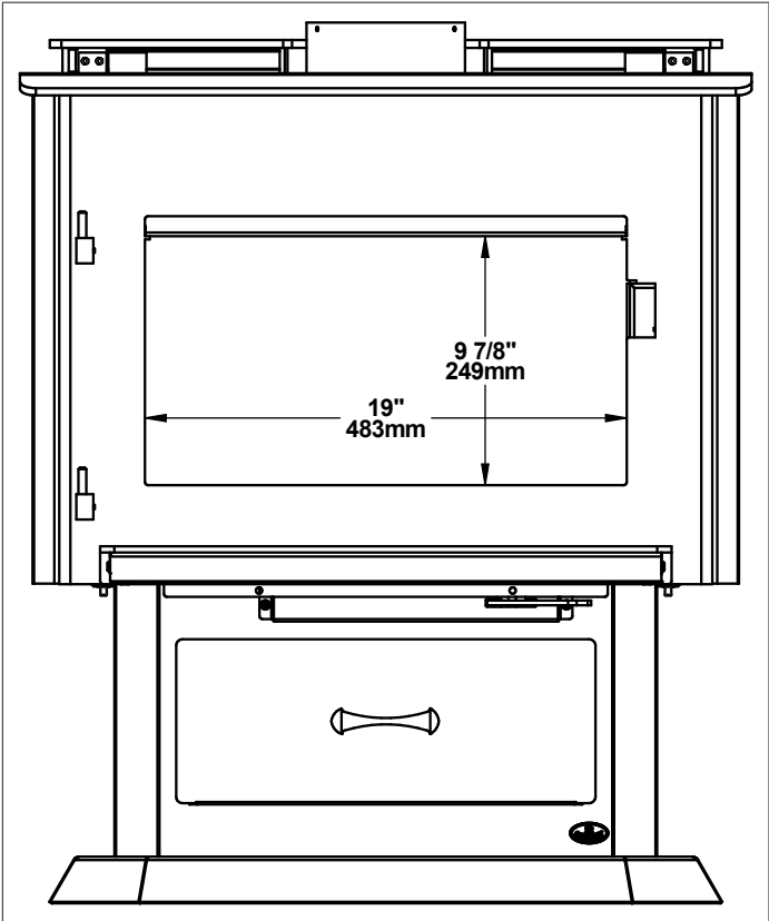
Figure 4: Door Opening
