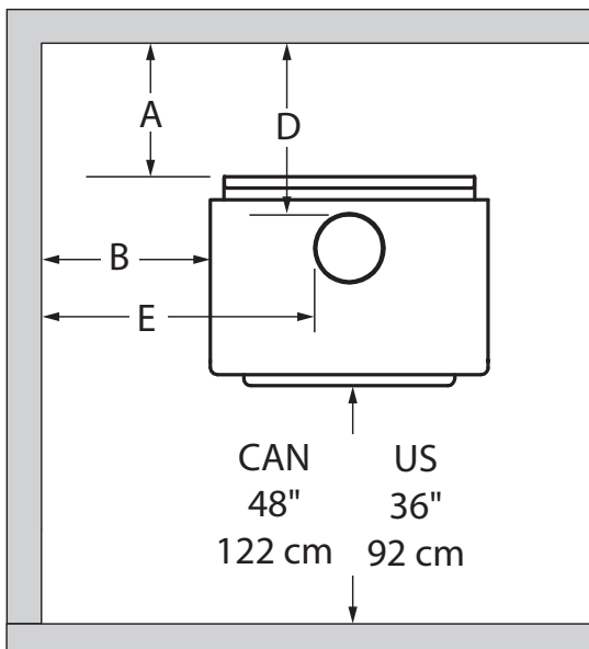
Figure 14: Clearances - Top
