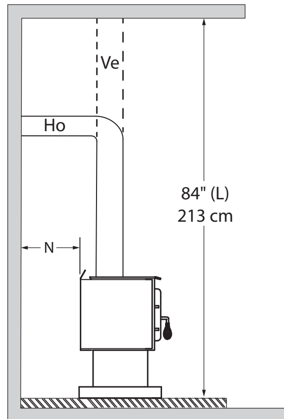
Figure 13: Clearances - Side
