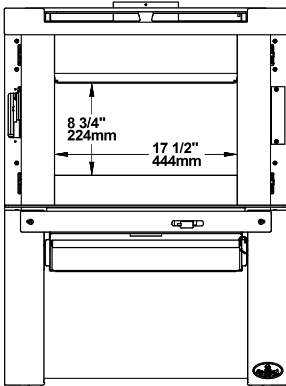
Figure 4: Door opening
