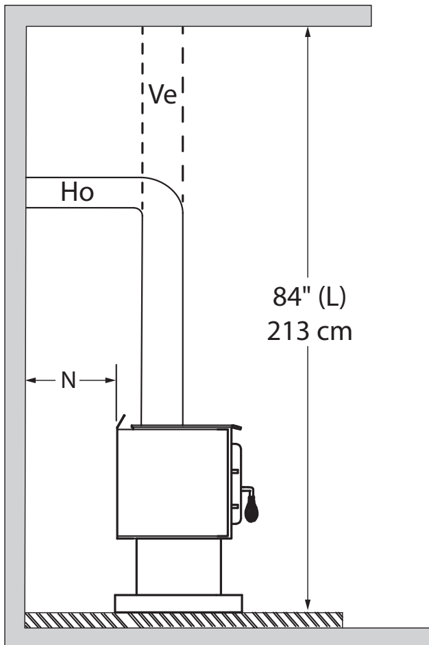
Figure 12: Clearances - Side
