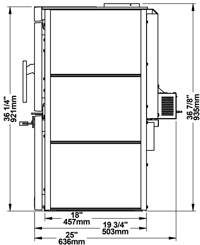
Figure 3: Side view
