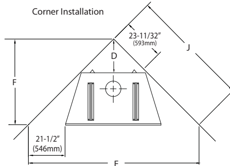
Back Wall of Chase/Enclosure Including Finishing Materials if any
