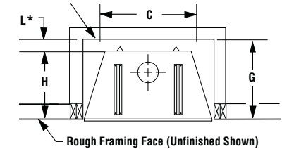
* Zero Clearance From Back Spacer to Wall
