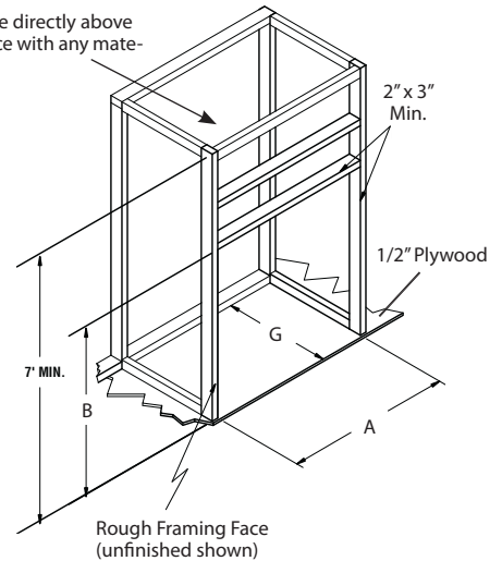
Back Wall of Chase/Enclosure Including Finishing Materials if any
